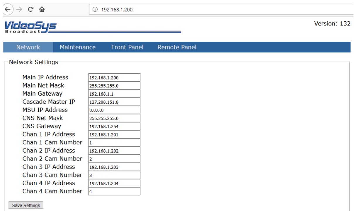
Fig 4. The IDUs Network Configuration Webpage
