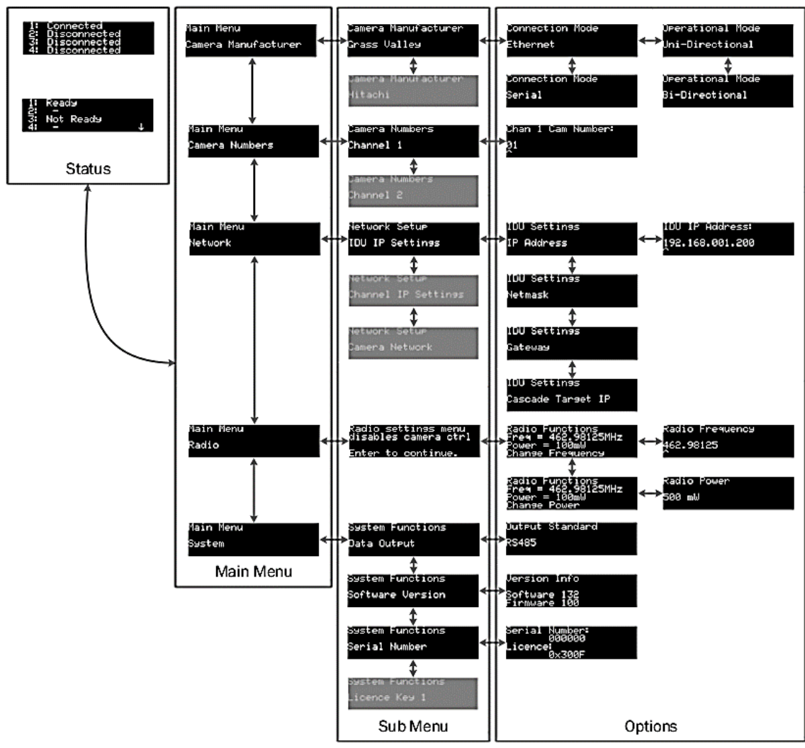
Fig 3. IDU menu structure diagram
