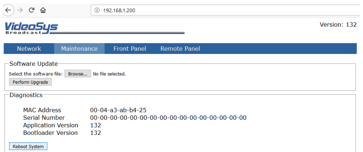
Fig 5. The IDUs Maintenance Webpage
