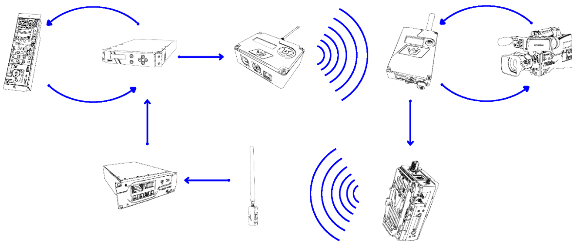
Fig 2. A simple bi-directional camera control setup utilising return via videolink data path
